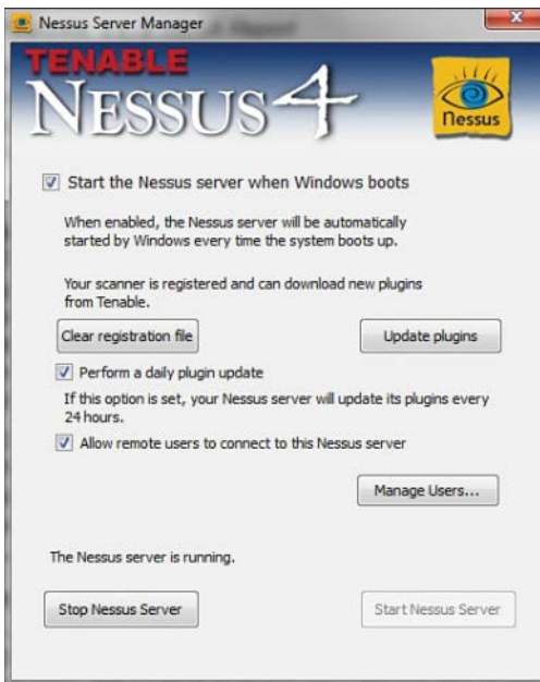
FIGURE 11.8 Nessus plugins.
